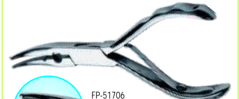
FP-51706 Fishing Pliers Chain Bent Grooved Jaws & Side Cutting 140mm, Polished Handles with Spring, Stainless Steel Made.
